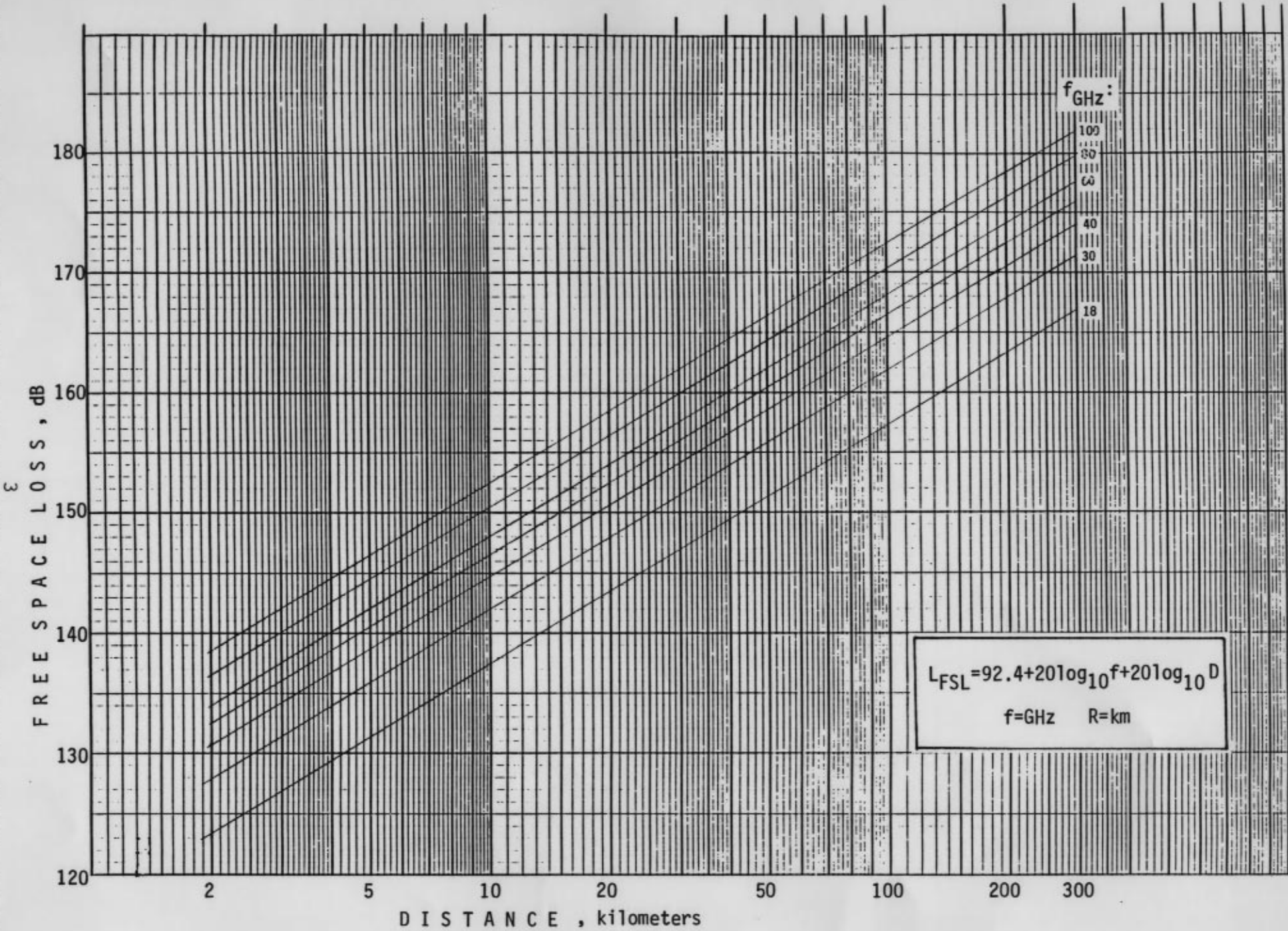
Figure 1: Free Space Loss Between Isotropic Antennas
