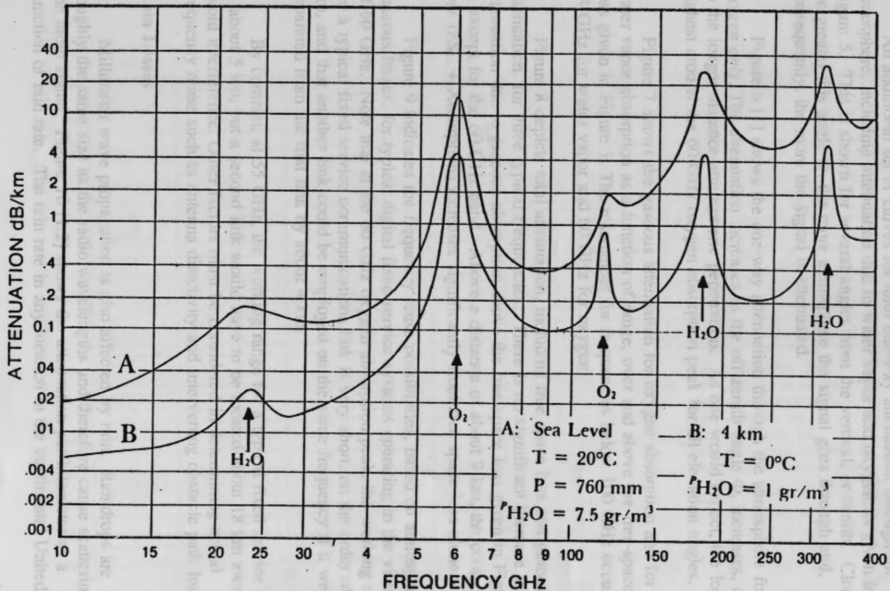
Figure 4: Average Atmospheric Absorption of Millimeter Waves.
