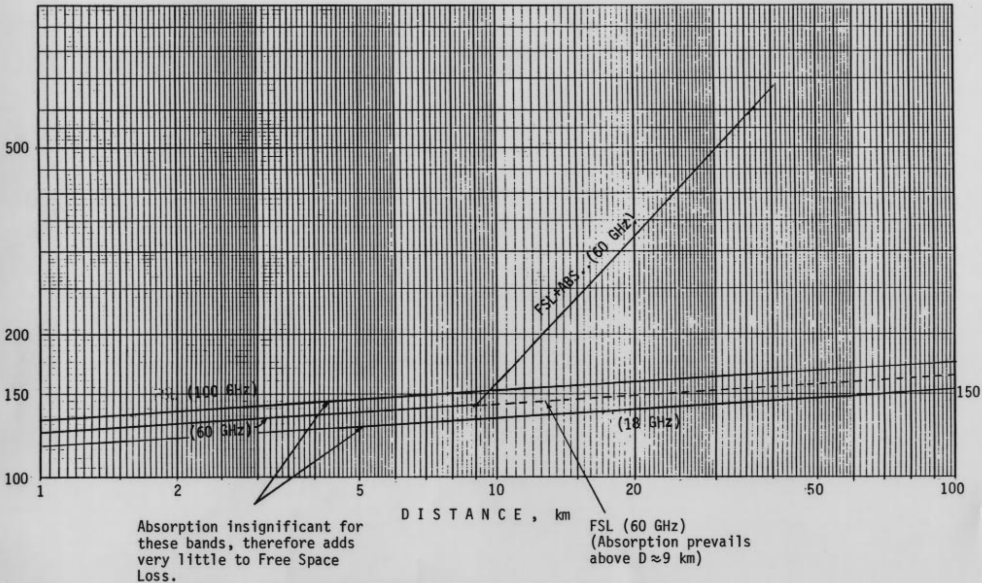
Figure 8: Combination Free Space Loss Plus Absorption.
